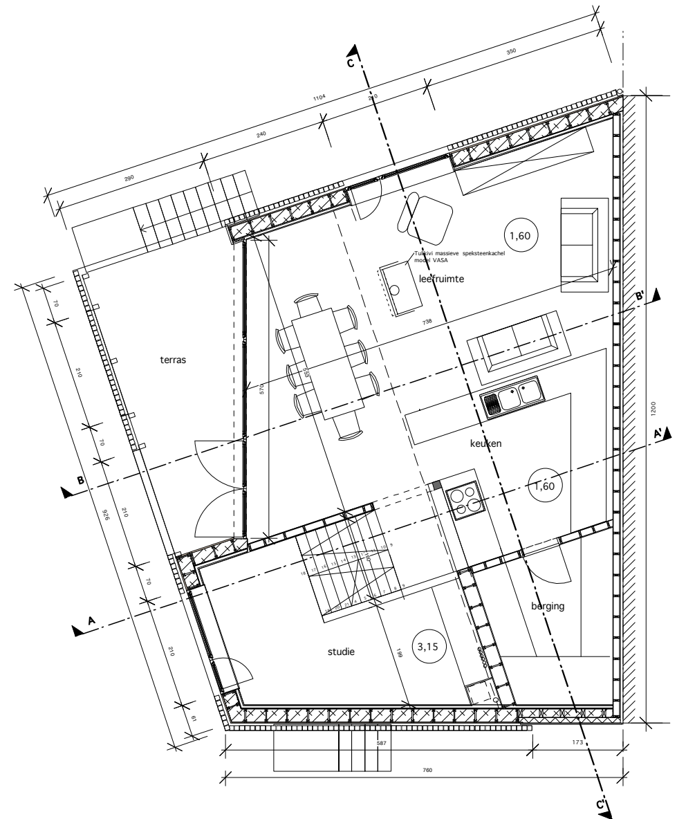
woning Dekeyzer 02 BEL-ETAGE schaal 1/100
