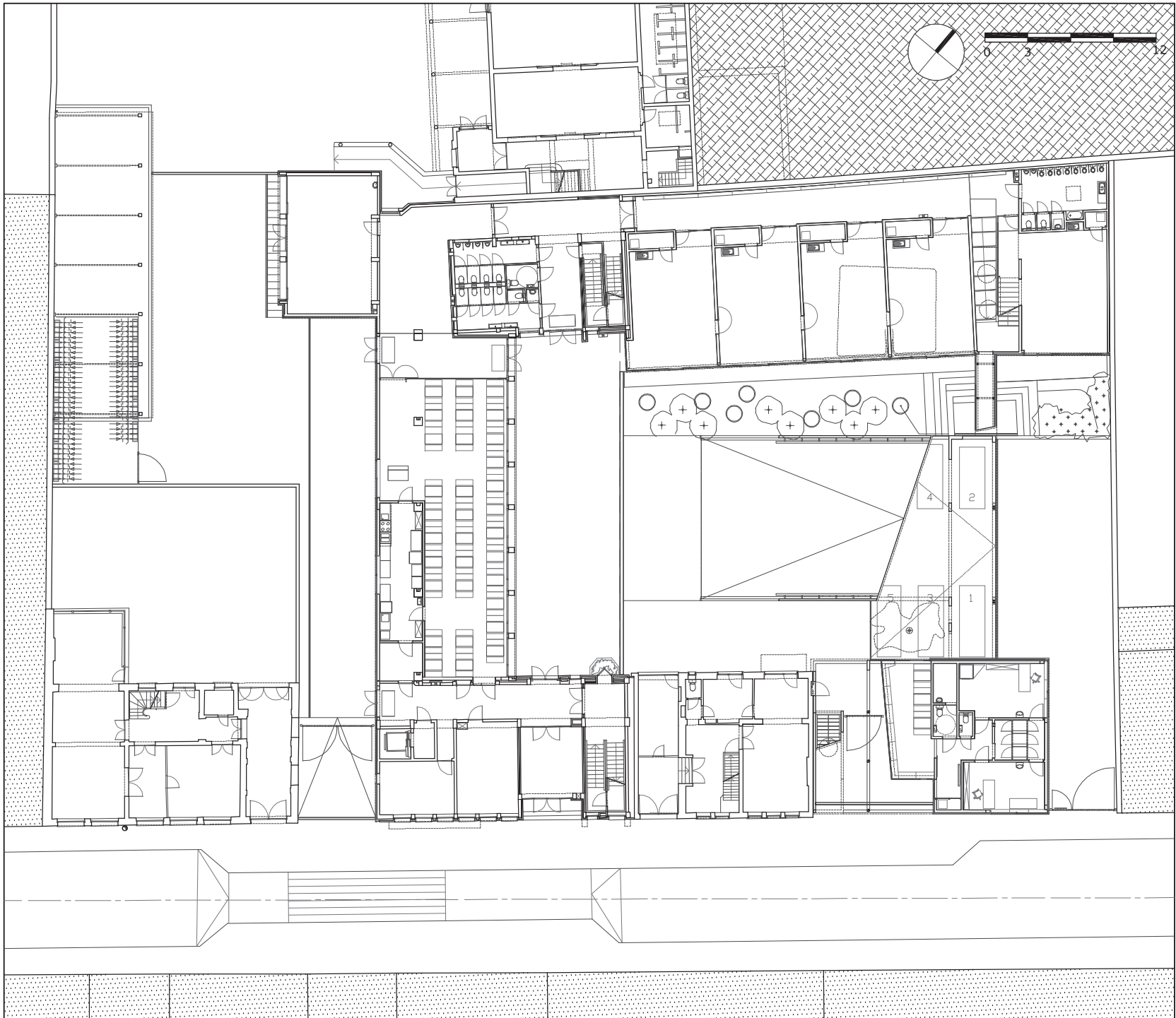
plan begane grond
