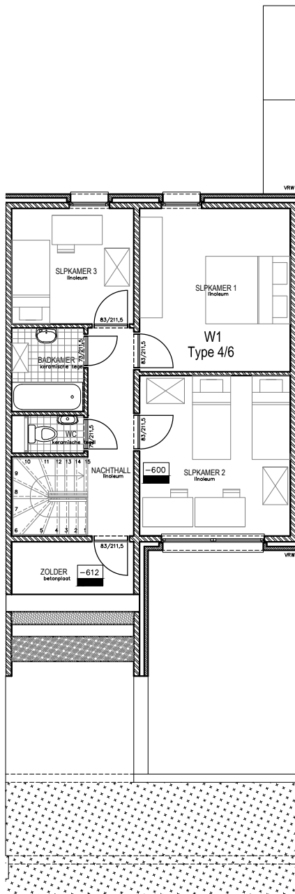
PLAN + SNEDE WONINGTYPE 4/6 \uparrow 1/100 PLAN 3 | Woonpunt Zennevallei Rodenem Halle | A2D architects
