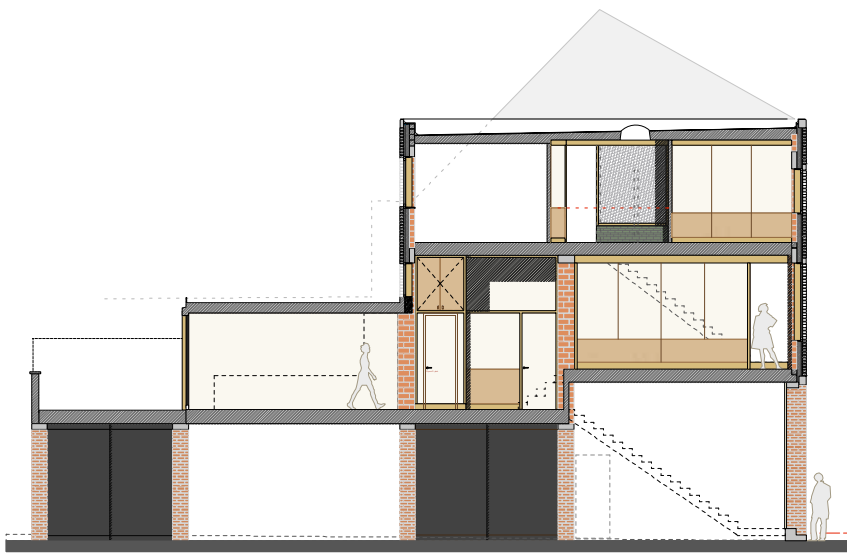
doorsnede over poortwoning
