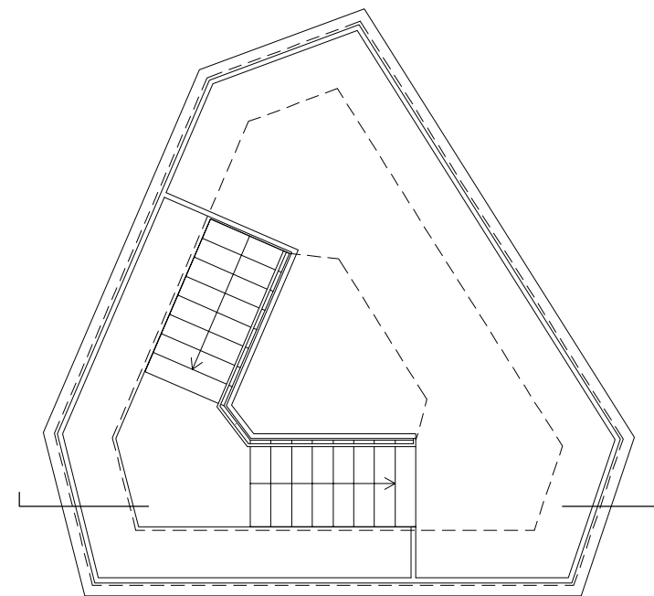
N ⊕ NIV +10.80m=48.00m TAW
