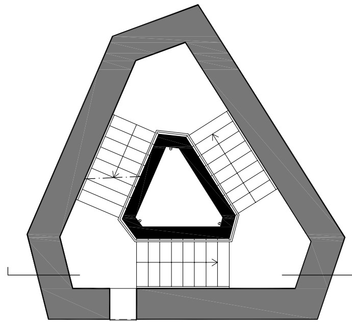
N ⊕ NIV +4.05m=41.25m TAW
