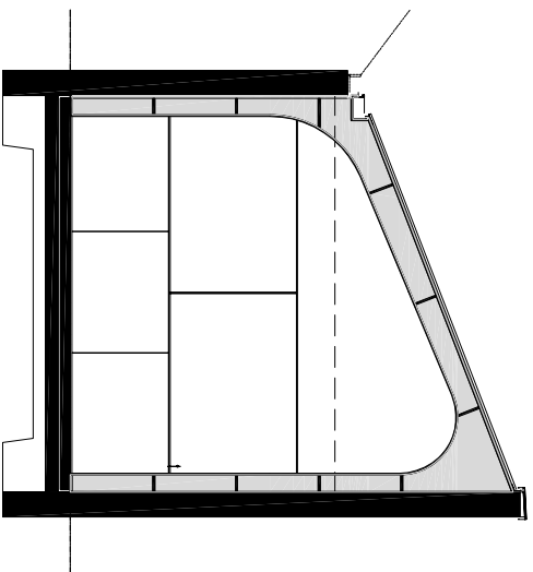
sneede B-B scale 1/100
