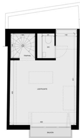
PLAN VERDEPING 2
