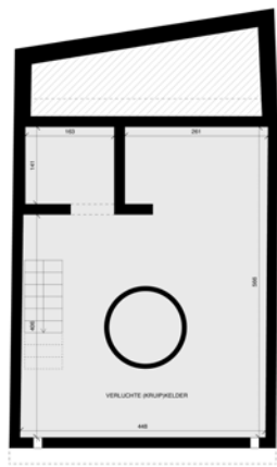
PLAN VERDEPING -1
