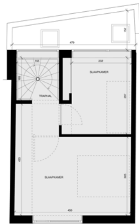
PLAN VERDEPING 1
