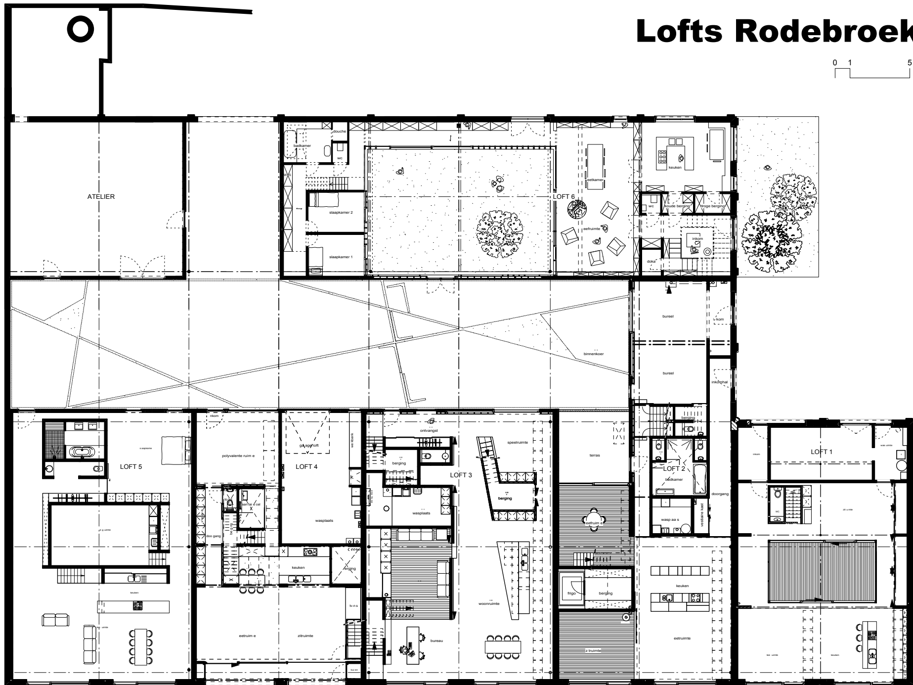
Plan begane grond
