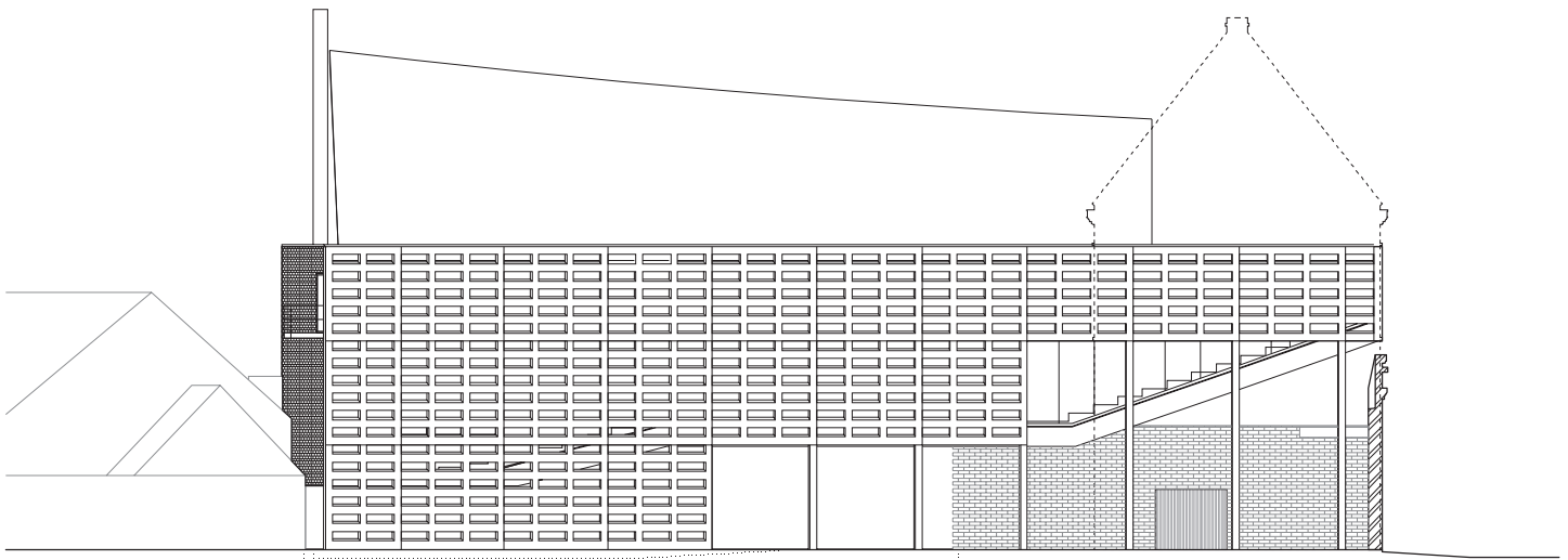
SOUTH FACADEN2 0 1 5
