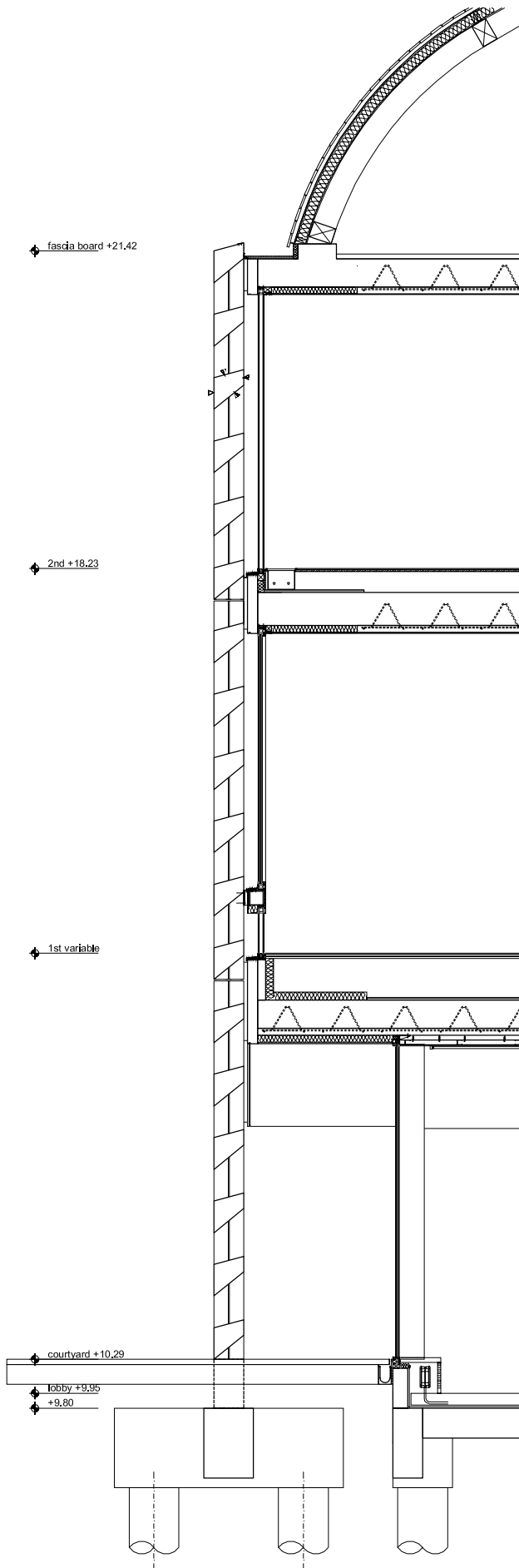
N2 SOUTH FAÇADE SECTION
